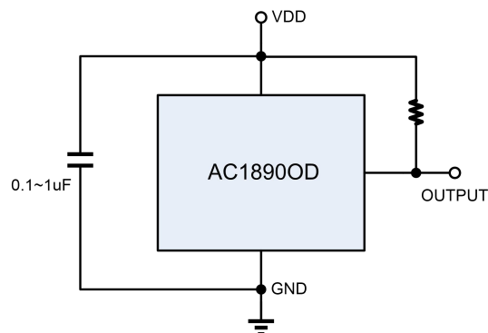
Figure 1, Typical Application Circuit of AS1890OD
