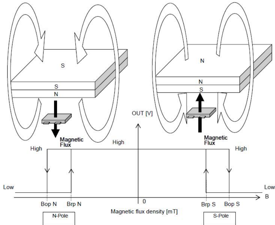
Fig 4, Magnetic Operation Characteristic of AS1890OD
