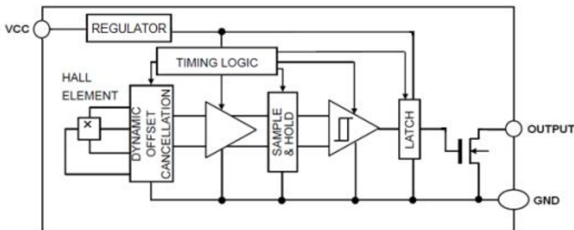
Figure2, Block Diagram of AS1890OD
